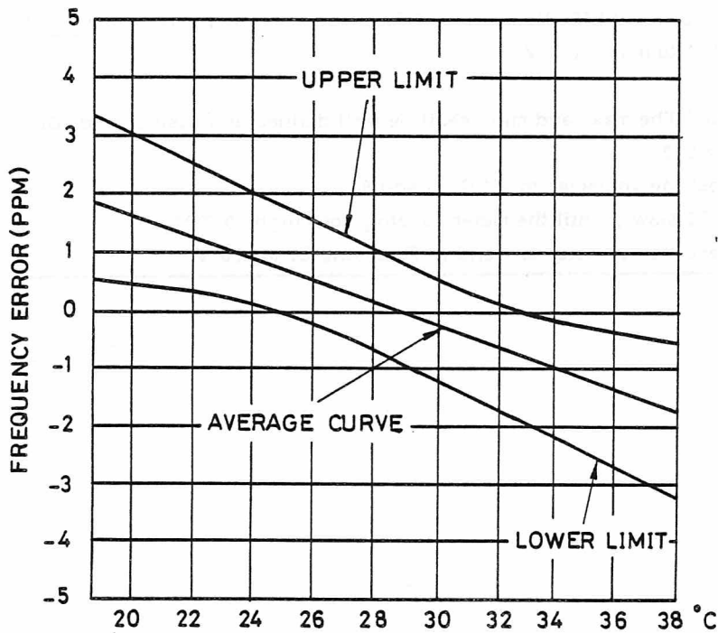
X0900 FREQUENCY ERROR CURVE
