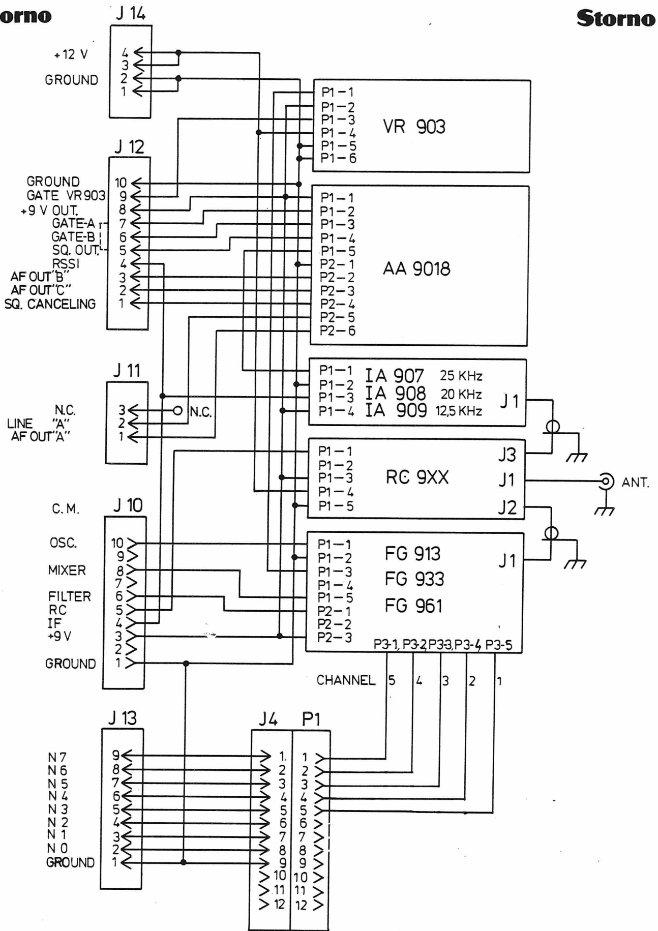
INTERCONNECTION DIAGRAM CQF9XXX RECEIVER WITH MULTIPLIER
