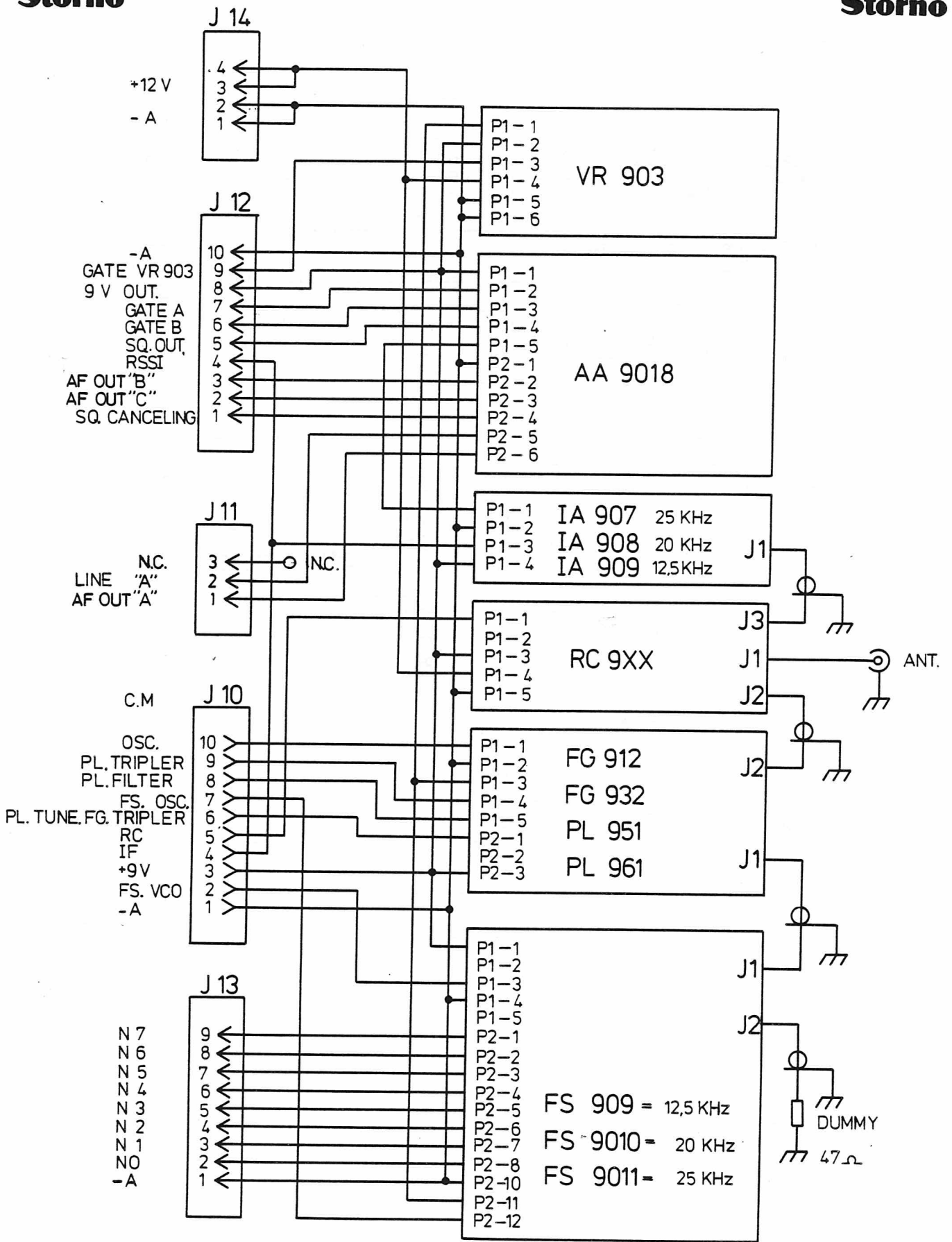
INTERCONNECTION DIAGRAM CQF9XXX RECEIVER WITH SYNTHESIZER
